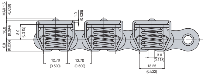
RS08BNPKUTS Gripper Chain™
