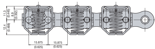
RS08BNPKUTS Gripper Chain™
