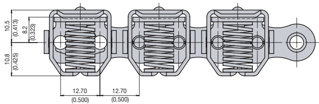
RS10BNPKUTM Gripper Chain™
